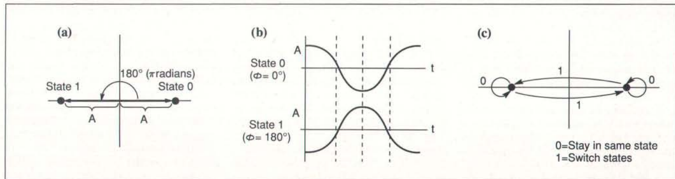
Figure 1: The states and transitions for a two-state differential phase-shift keying modulation scheme. (a) The amplitude, which is the same for all states in PSK, is represented by the length of the line joining each point to the origin, while the phase is represented by the angle of that line relative to the positive half of the horizontal axis. (b) Two carrier signals that have the same shape but are 180° out of phase. (c) A possible way of encoding 1 and 0 bits as transitions between the states.
